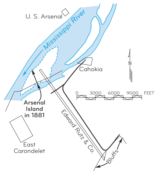
Figure 8-106. The record location of the Rutz property at the time of trial extended onto the new location of Arenal Island.
