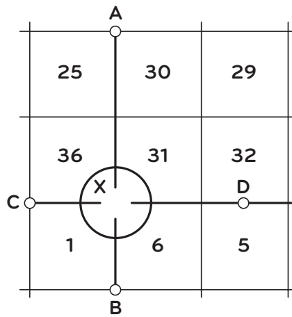
Lost township corner in vicinity of X.
